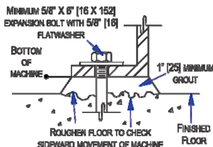
ANCHORING DETAIL
