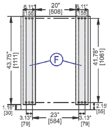
FOUNDATION PLAN
