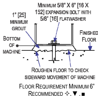
ANCHORING DETAIL
